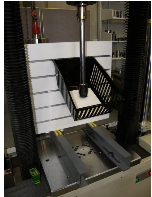
FIG.2. TEST SET-UP
