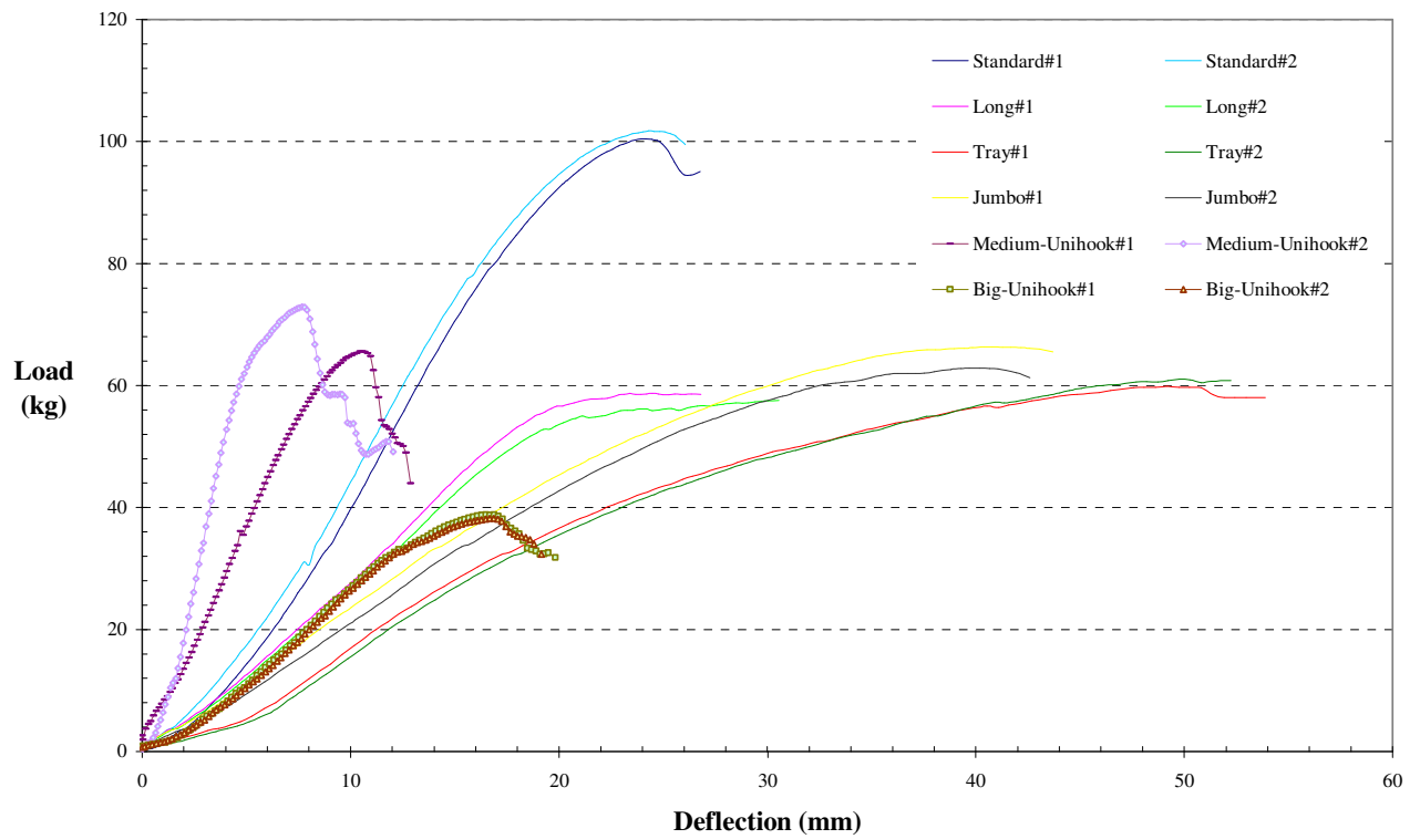
CRATEBOX™ LOAD VS DEFLECTION CURVES FIG A1
